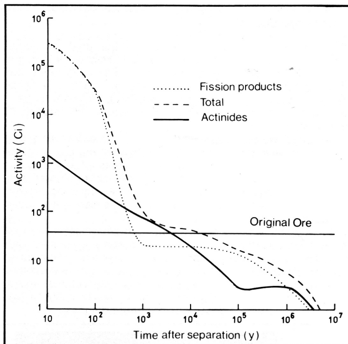
Activity of waste from 1t fuel and its originating ore body.
