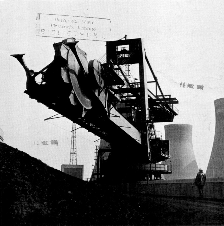
“A stocking-out and coal-reclaiming machine at the 1980 MW coal-fired Drax power station, in Yorkshire”
