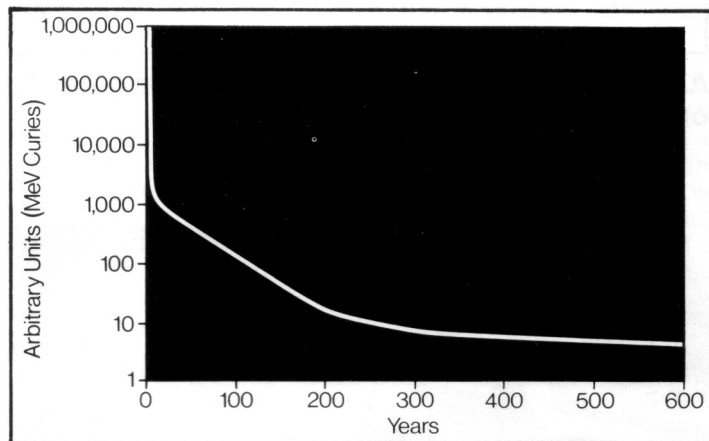
Decay in activity of waste constituents in spent 'Magnox' fuel.
